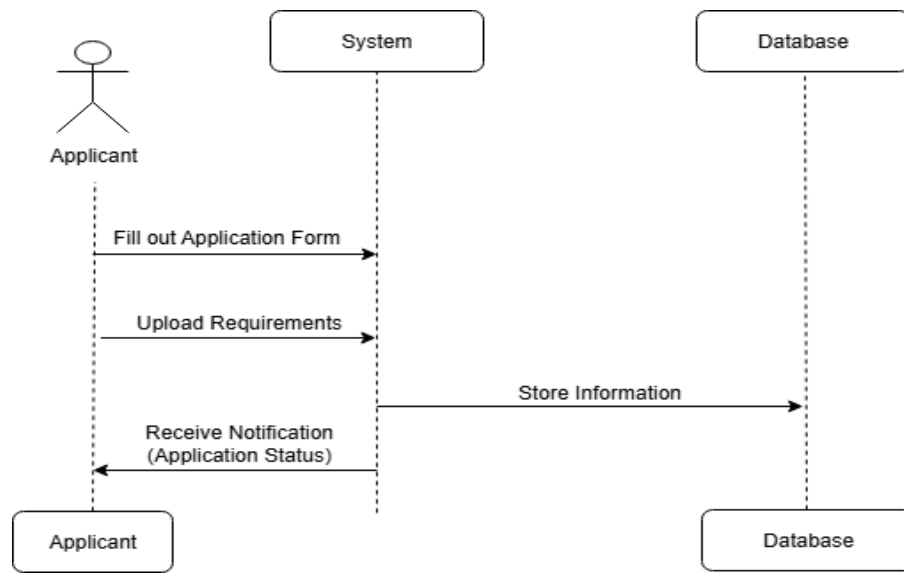
Figure 9. Sequence Diagram - Applicants
