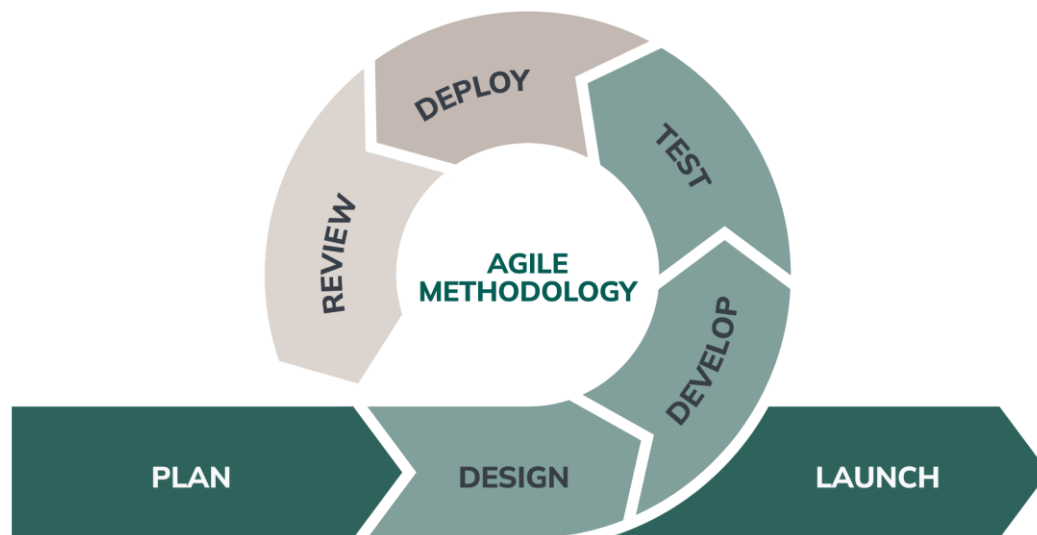
Figure 1. Agile Methodology
