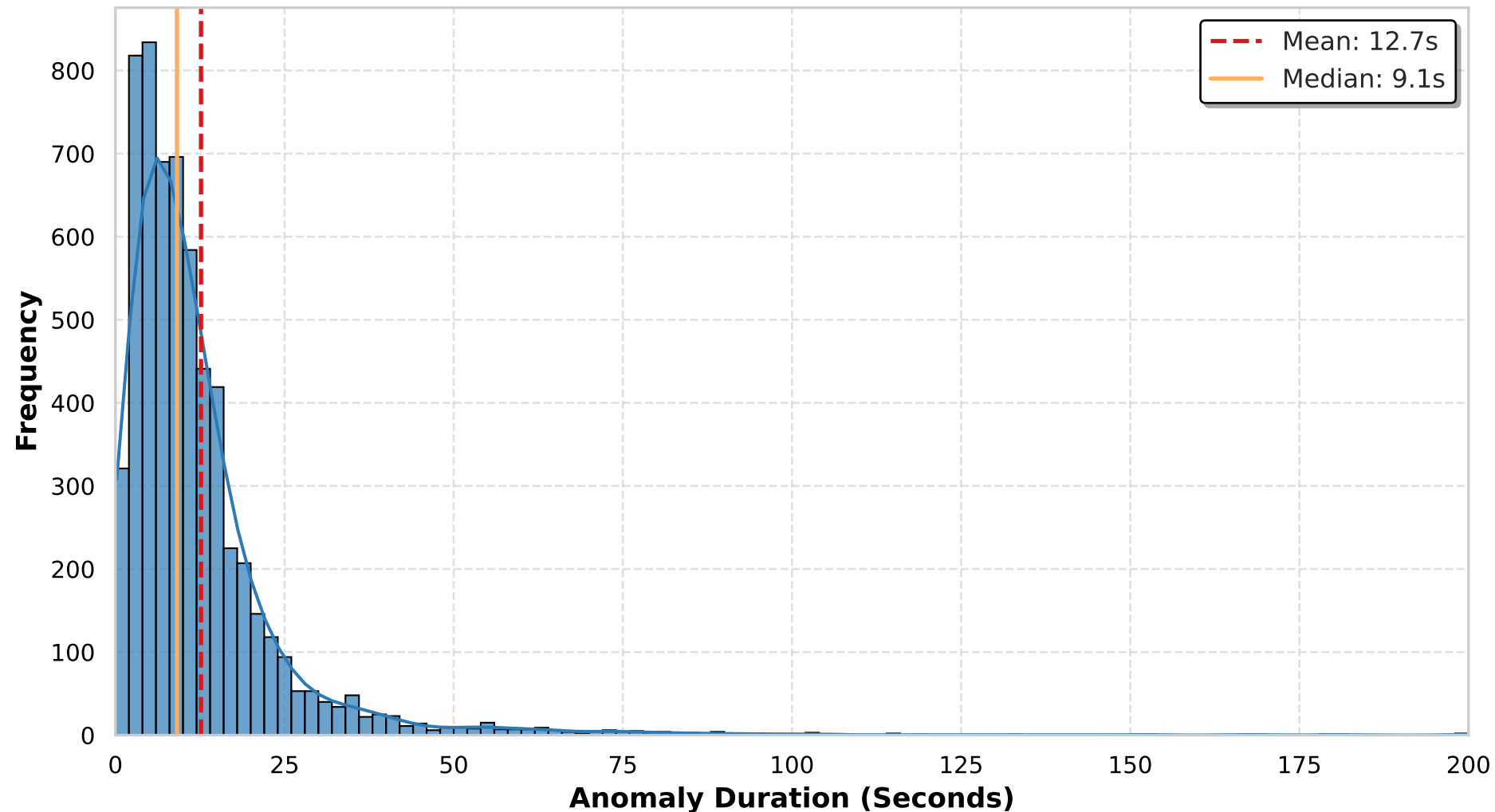
Distribution of Anomaly Durations in the UCF-Crime Train Split
