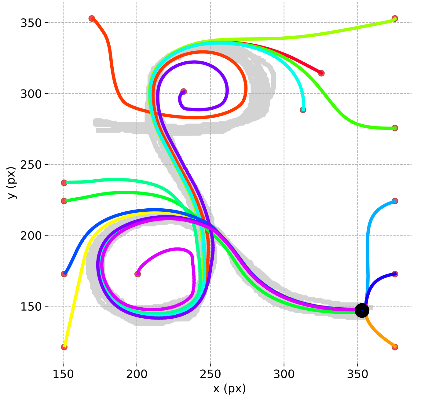
Dynamic system with CONDOR framework latent dim 256
