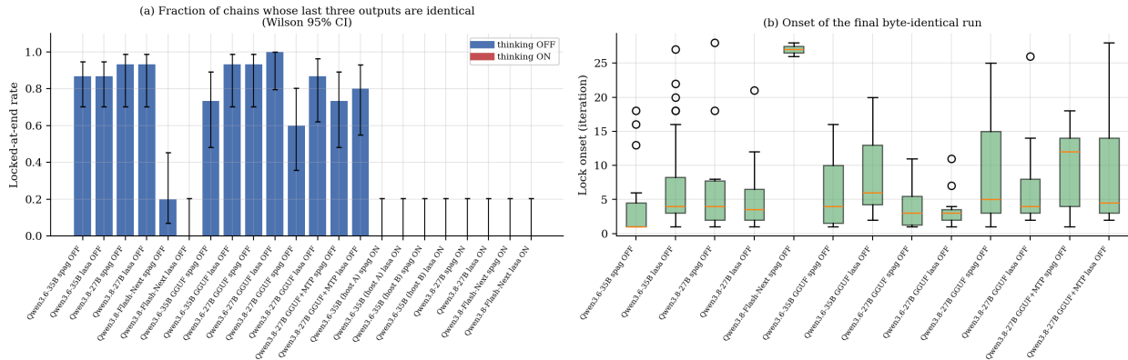
Figure 9: Locked-at-end rate with Wilson intervals, and lock-onset distribution, per configuration and recipe, thinking off and on.
