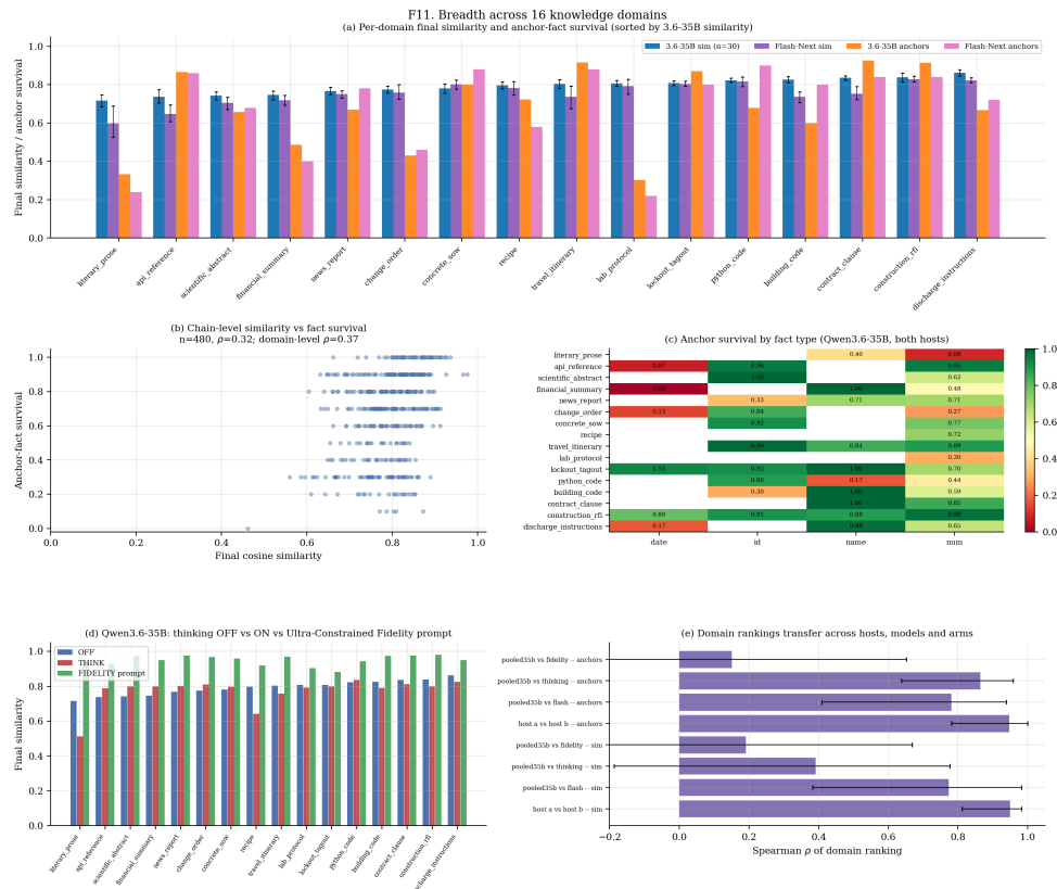
Figure 11: Sixteen domains on Qwen3.6-35B (30 samples per domain, both hosts) and Flash-Next (5). (a) Final similarity and anchor-factor survival per domain. (b) Similarity against survival per chain. (c) Survival by fact type. (d) Thinking off, thinking on, and the fidelity prompt per domain. (e) Domain rankings transfer across hosts, models and arms.
