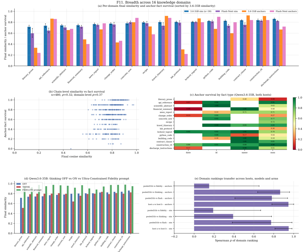
Figure 11: Sixteen domains on Qwen3.6-35B (30 samples per domain, both hosts) and Flash-Next (5). (a) Final similarity and anchor-fact survival per domain. (b) Similarity against survival per chain. (c) Survival by fact type. (d) Thinking off, thinking on, and the fidelity prompt per domain. (e) Domain rankings transfer across hosts, models and arms.
