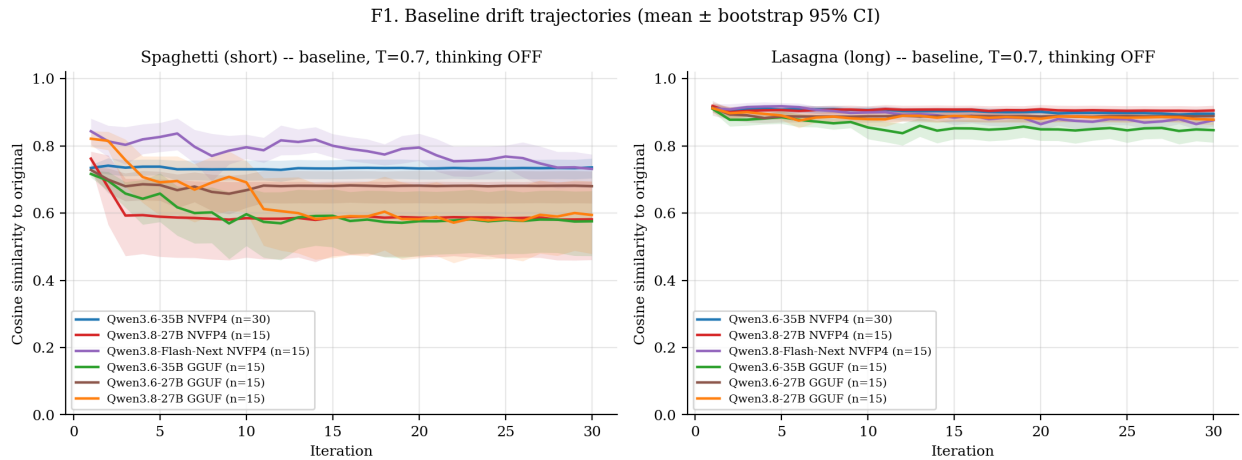
Figure 1: Baseline drift trajectories for the six non-MTP configurations, mean with bootstrap band; n in the legend. Left: spaghetti. Right: lasagna.
