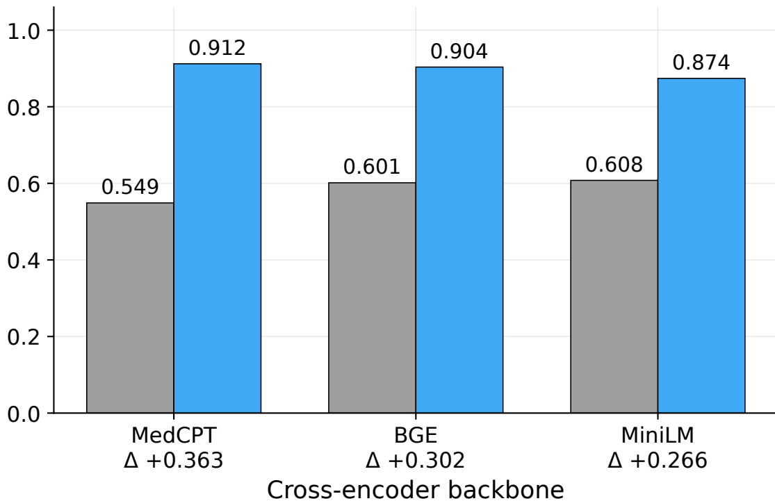
Validation Dev Recall@5
