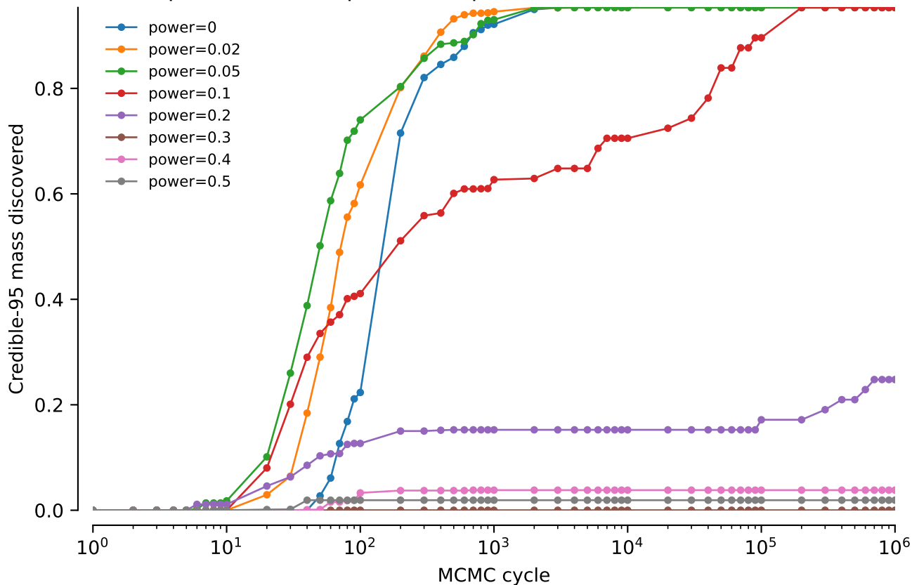
vert.atpase6.tw0: NNI power comparison: Credible-95 mass discovered
