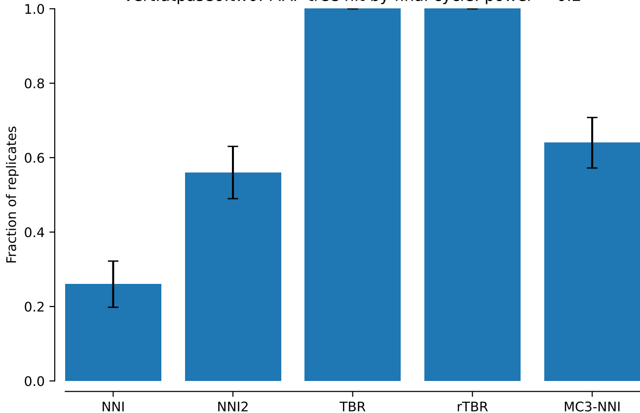
vert.atpase6.tw0: MAP tree hit by final cycle: power = 0.2
