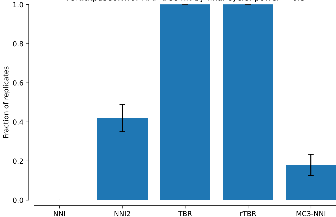
vert.atpase6.tw0: MAP tree hit by final cycle: power = 0.3
