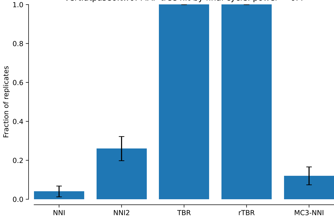
vert.atpase6.tw0: MAP tree hit by final cycle: power = 0.4
