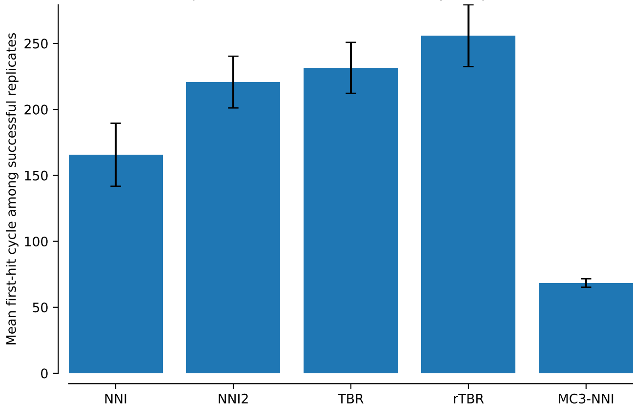
vert.atpase6.tw0: Mean MAP first-hit cycle: power = 0
