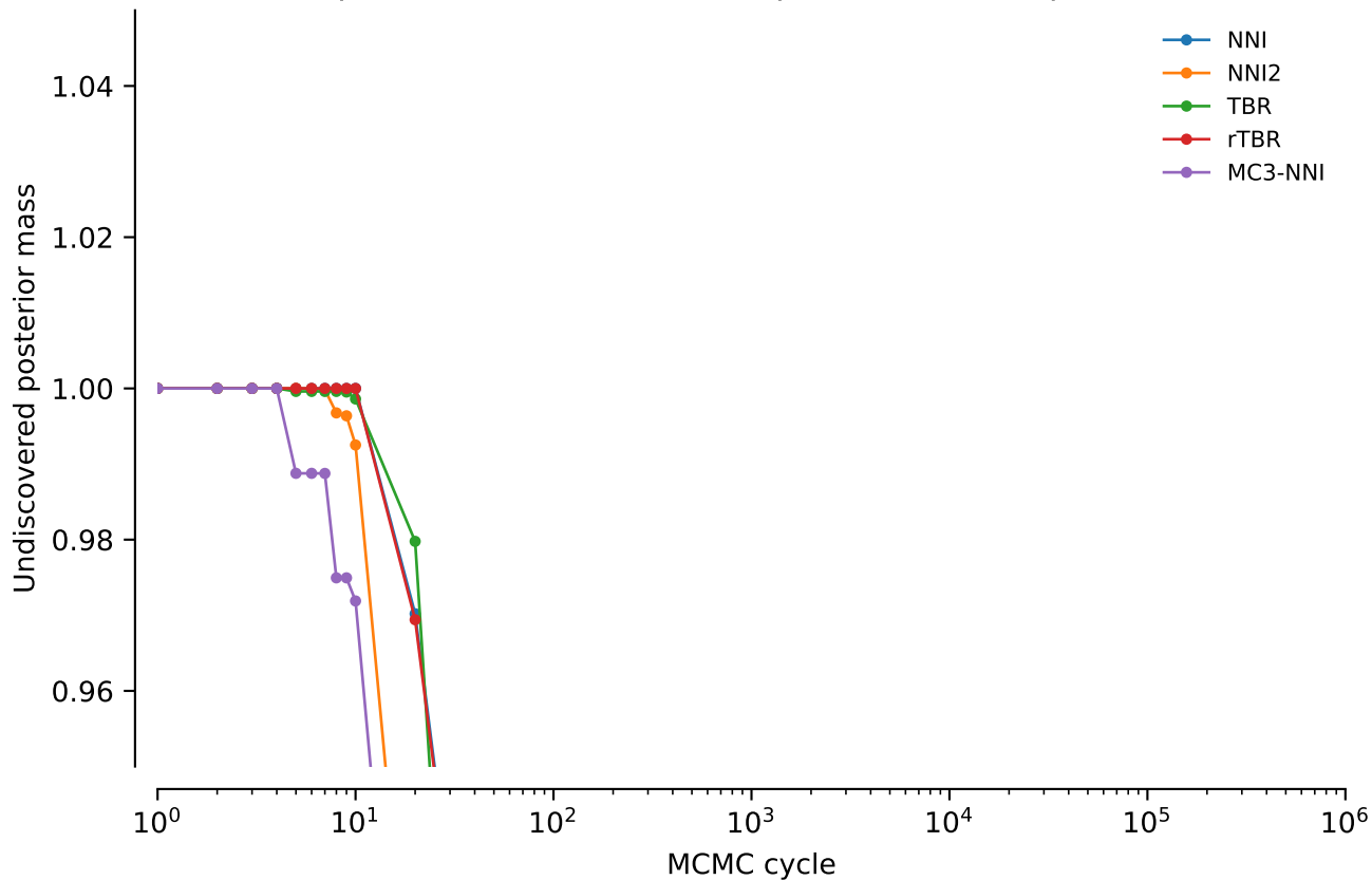
vert.atpase6.tw0: Undiscovered posterior mass: power = 0.02
