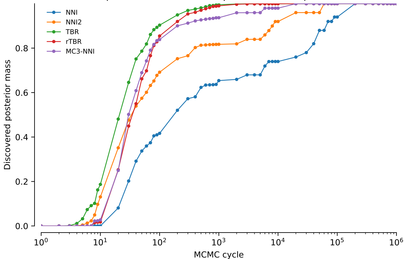
vert.atpase6.tw0: Discovered posterior mass: power = 0.1
