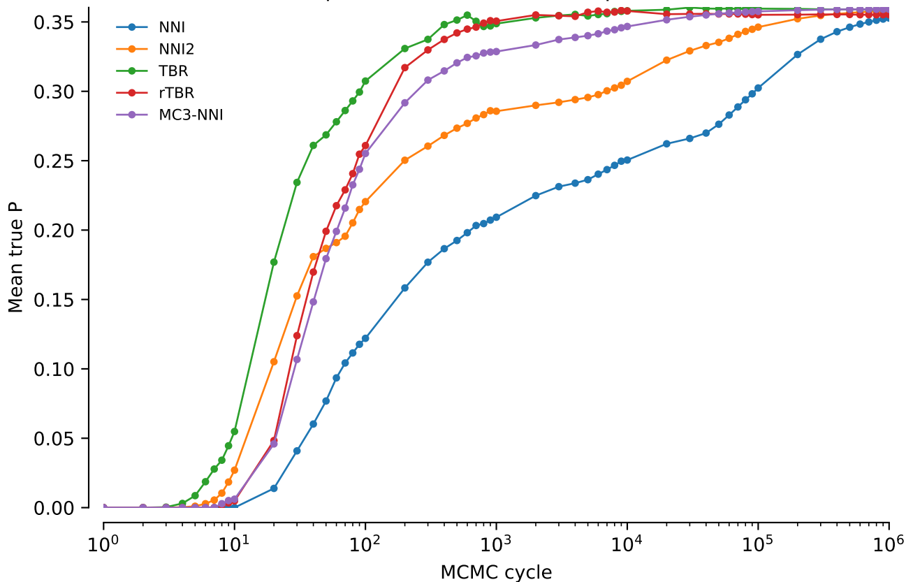
vert.atpase6.tw0: Mean true P: power = 0.1
