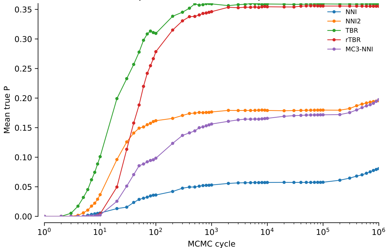
vert.atpase6.tw0: Mean true P: power = 0.2
