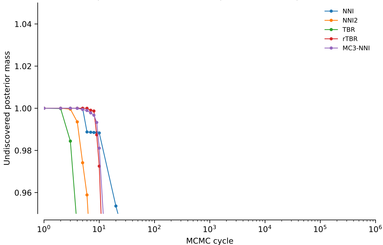
vert.atpase6.tw0: Undiscovered posterior mass: power = 0.2
