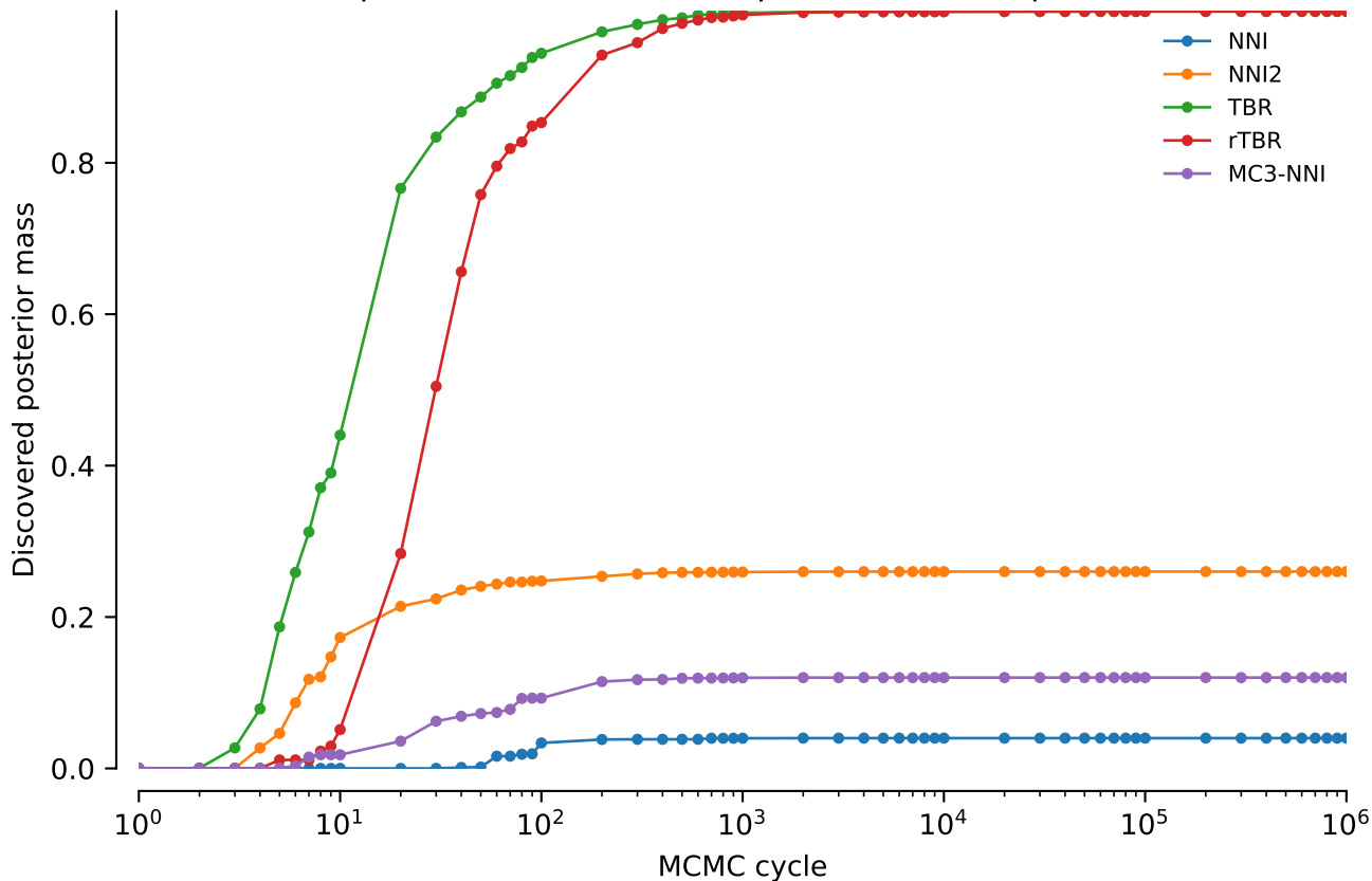
vert.atpase6.tw0: Discovered posterior mass: power = 0.4
