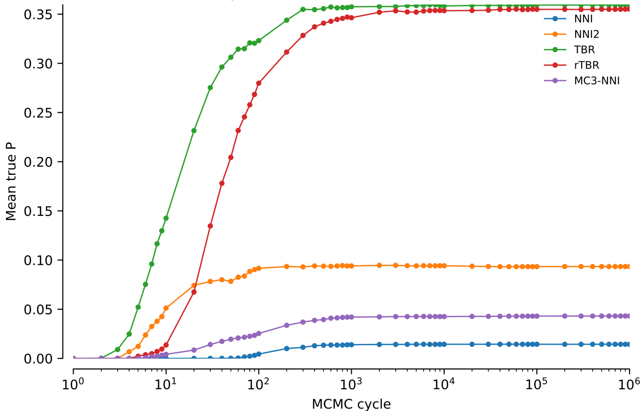
vert.atpase6.tw0: Mean true P: power = 0.4
