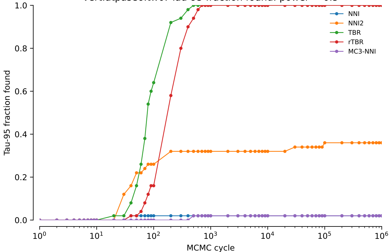
vert.atpase6.tw0: Tau-95 fraction found: power = 0.5
