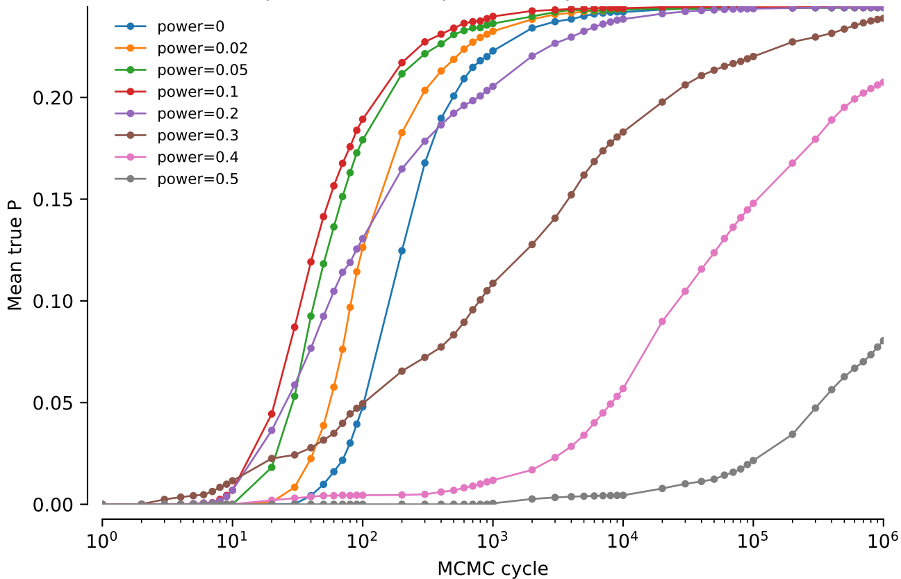
vert.atpase6.tw5: NNI power comparison: Mean true P
