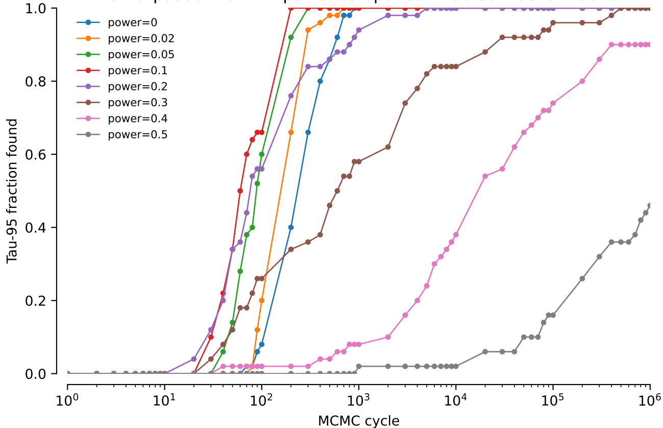
vert.atpase6.tw5: NNI power comparison: Tau-95 fraction found
