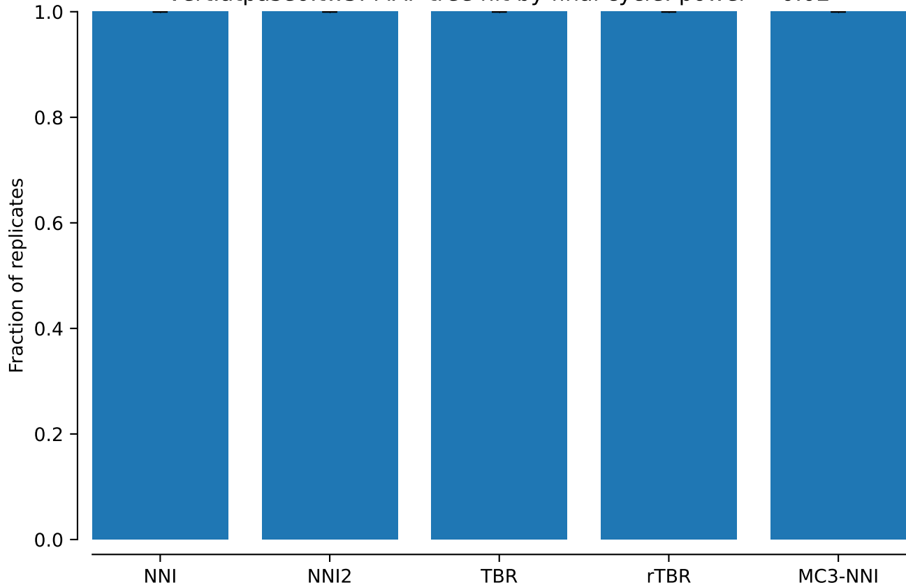
vert.atpase6.tw5: MAP tree hit by final cycle: power = 0.02
