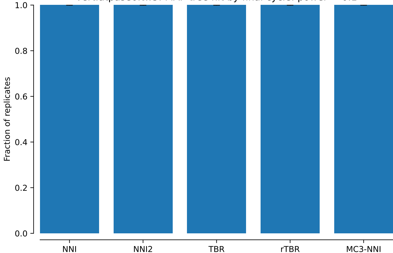
vert.atpase6.tw5: MAP tree hit by final cycle: power = 0.1
