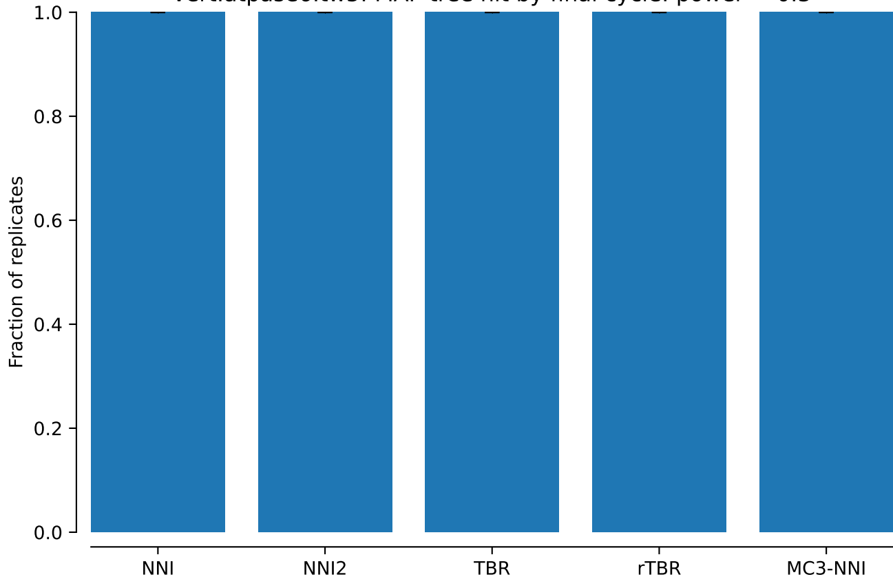
vert.atpase6.tw5: MAP tree hit by final cycle: power = 0.3
