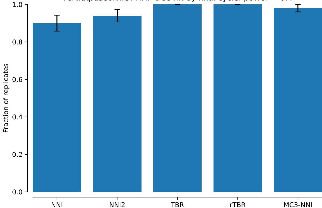
vert.atpase6.tw5: MAP tree hit by final cycle: power = 0.4
