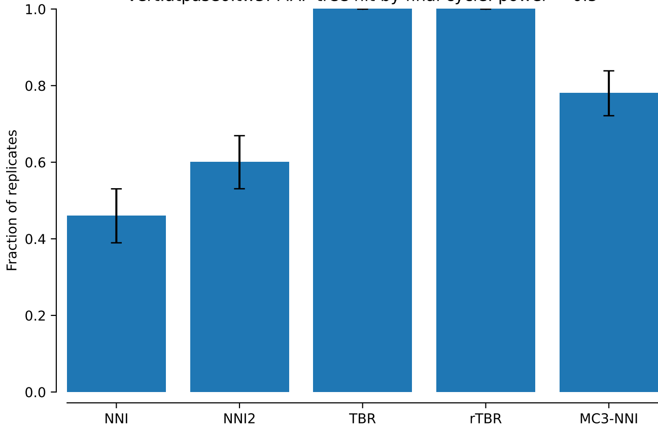
vert.atpase6.tw5: MAP tree hit by final cycle: power = 0.5
