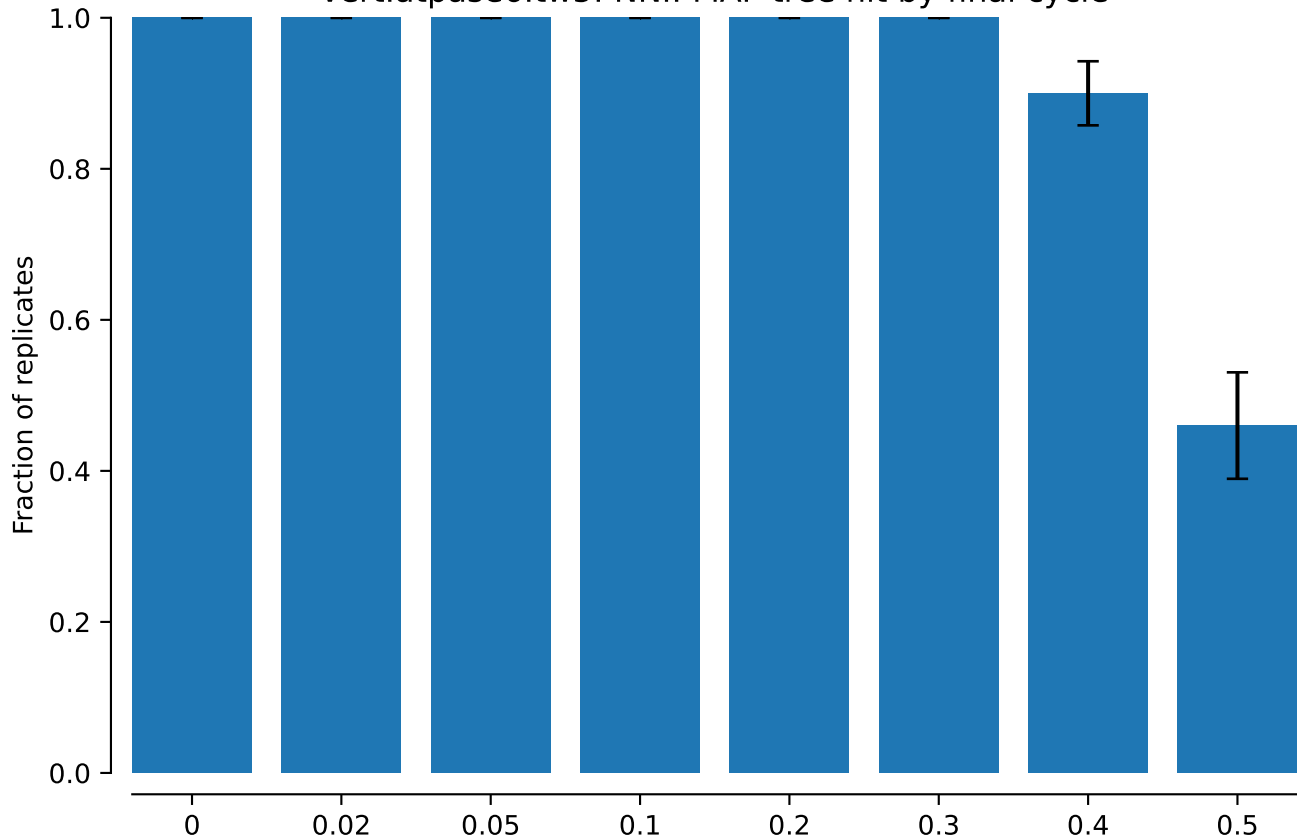
vert.atpase6.tw5: NNI: MAP tree hit by final cycle
