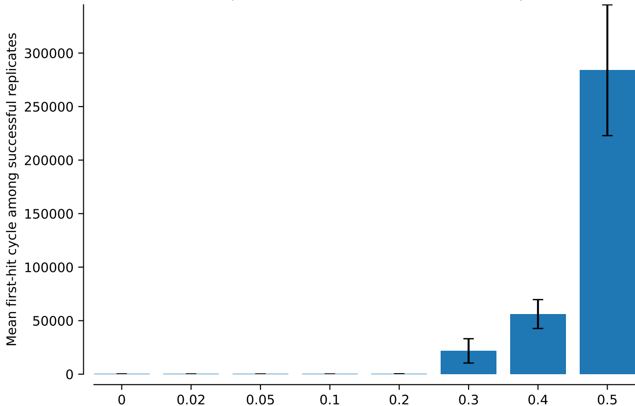
vert.atpase6.tw5: NNI: mean MAP first-hit cycle
