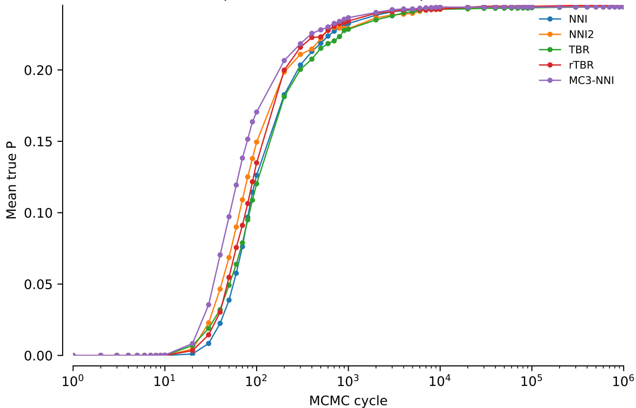
vert.atpase6.tw5: Mean true P: power = 0.02
