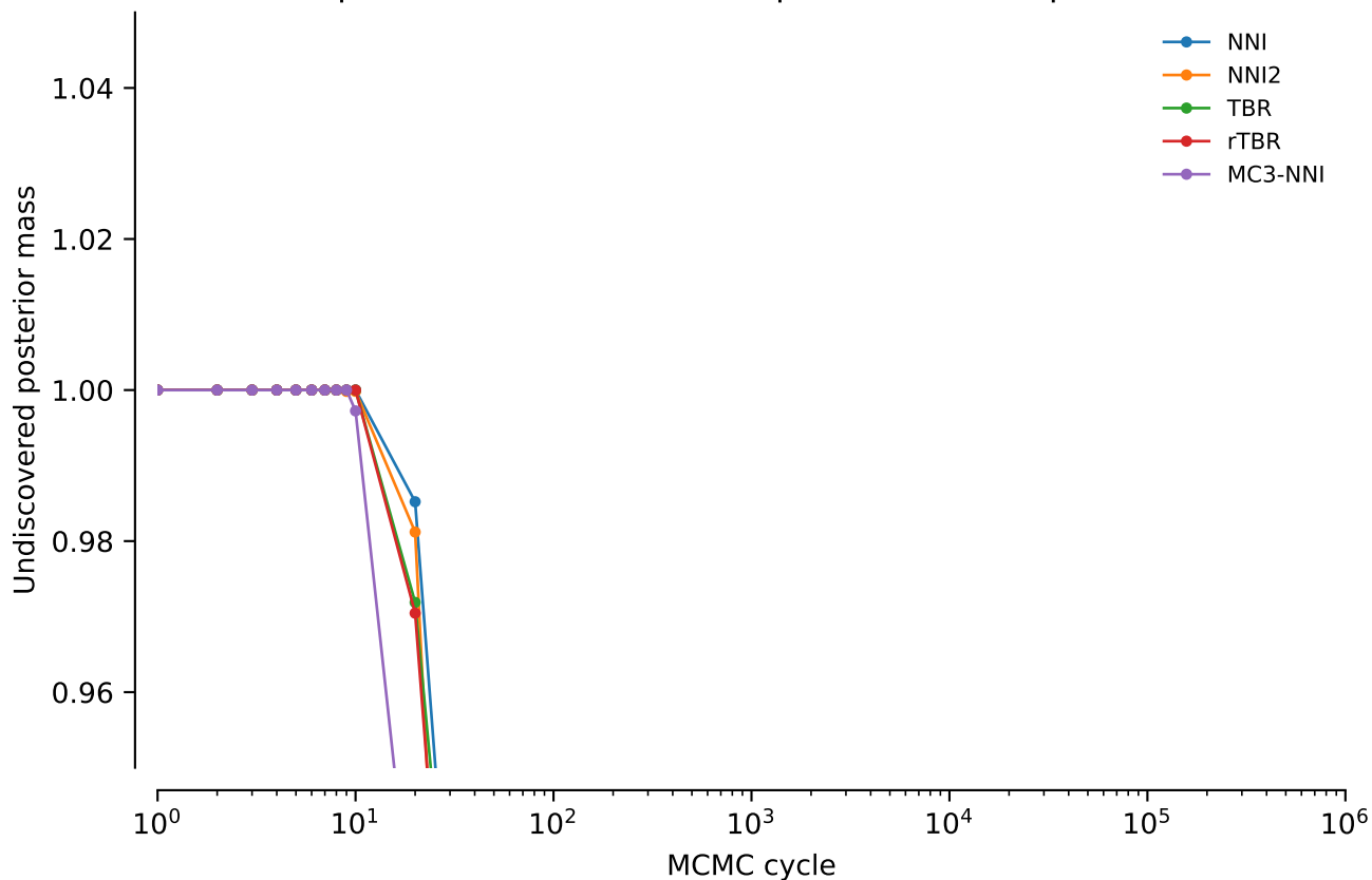
vert.atpase6.tw5: Undiscovered posterior mass: power = 0.02
