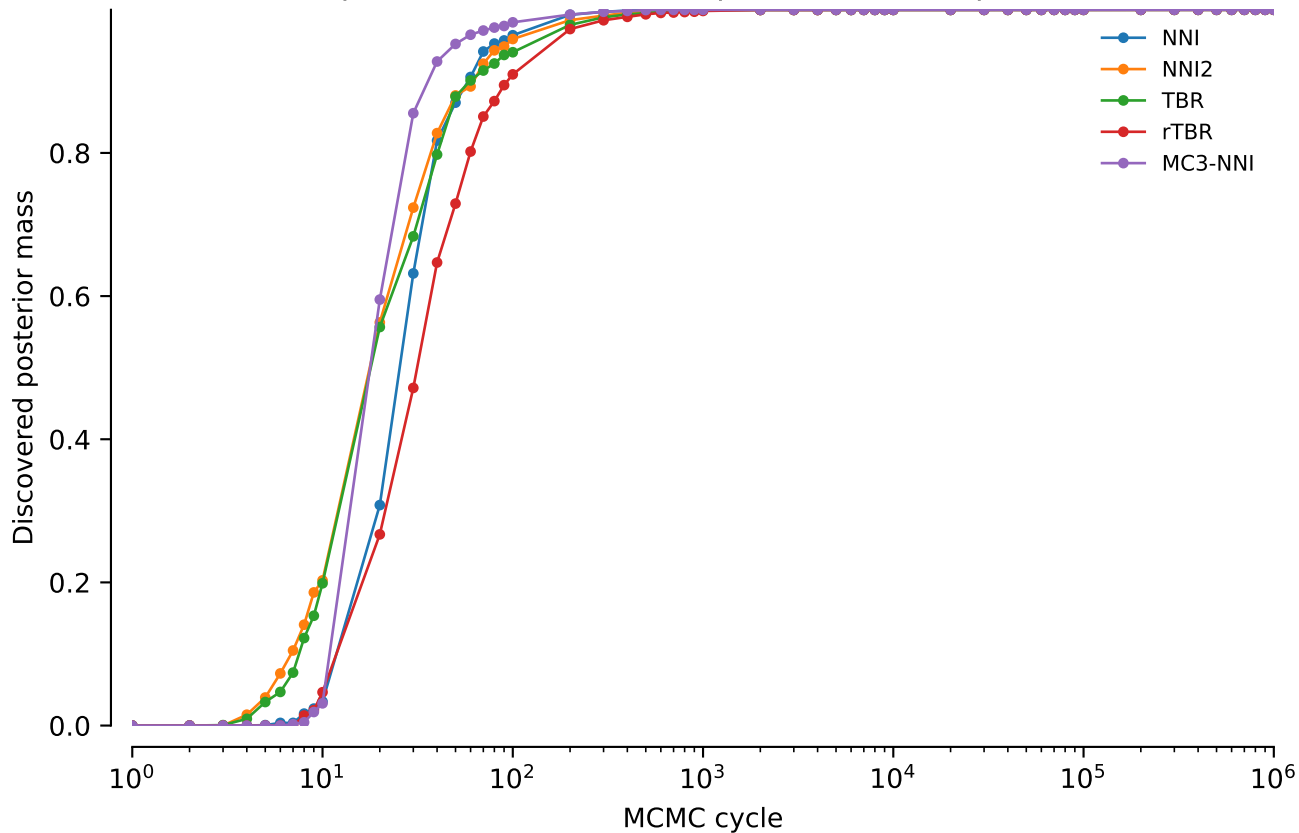
vert.atpase6.tw5: Discovered posterior mass: power = 0.1
