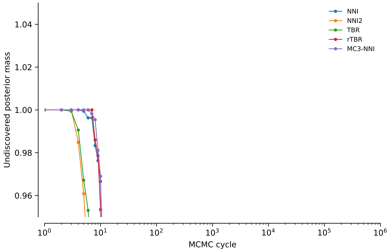
vert.atpase6.tw5: Undiscovered posterior mass: power = 0.1
