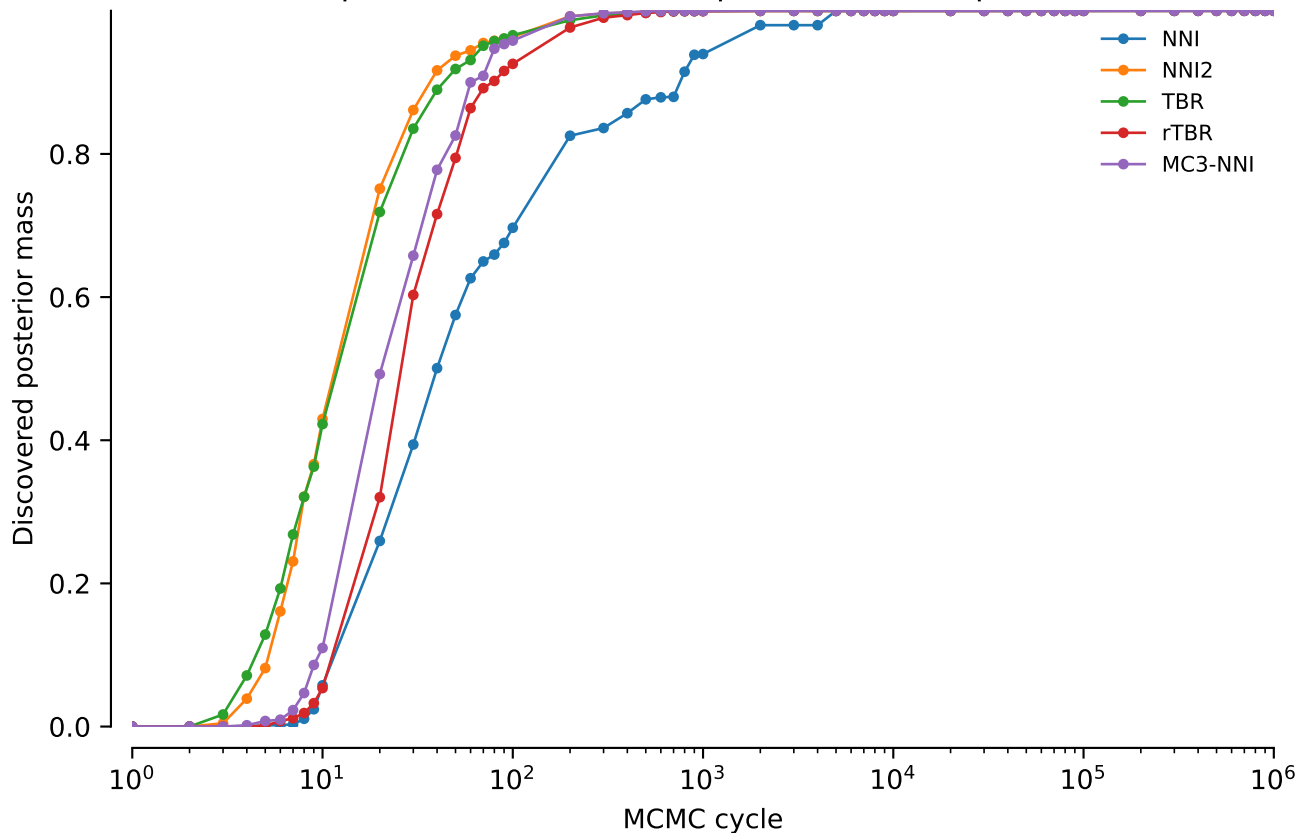
vert.atpase6.tw5: Discovered posterior mass: power = 0.2
