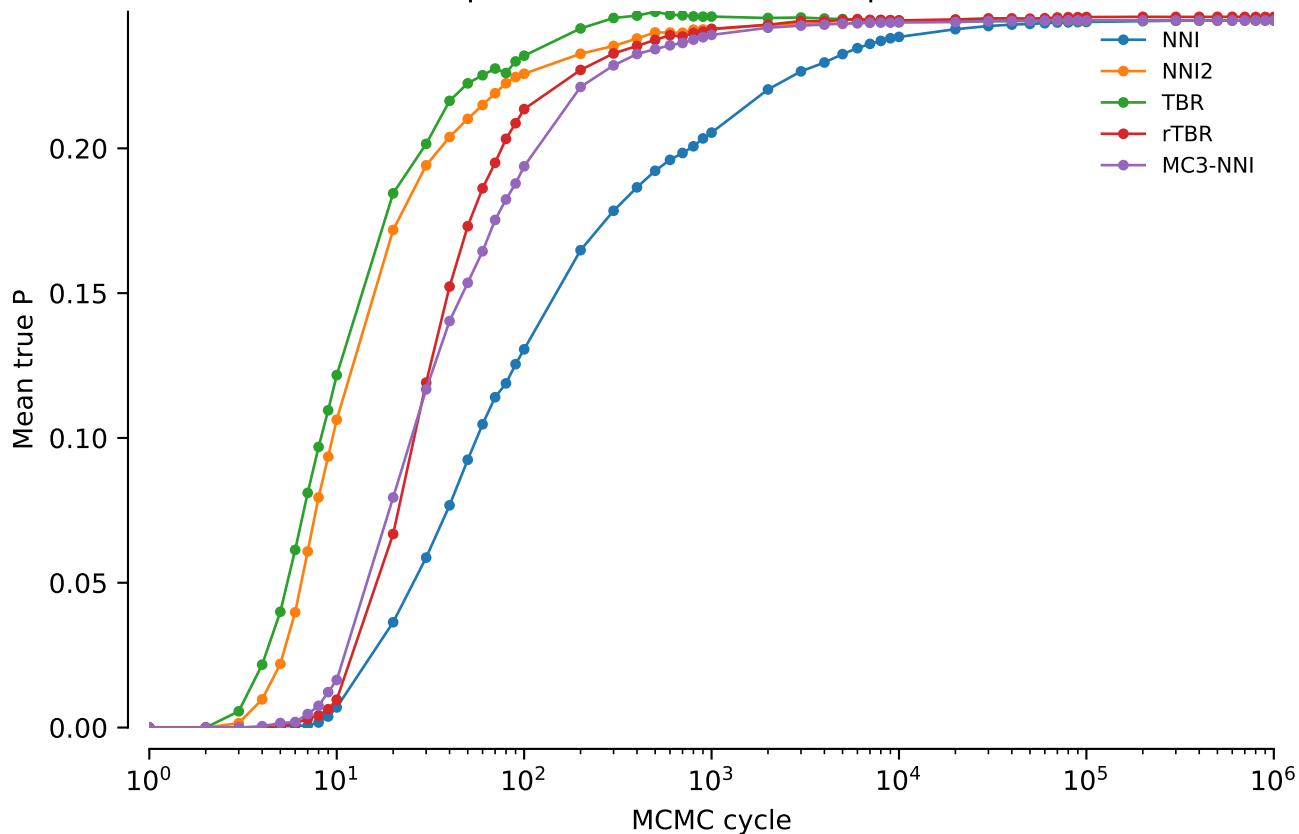
vert.atpase6.tw5: Mean true P: power = 0.2
