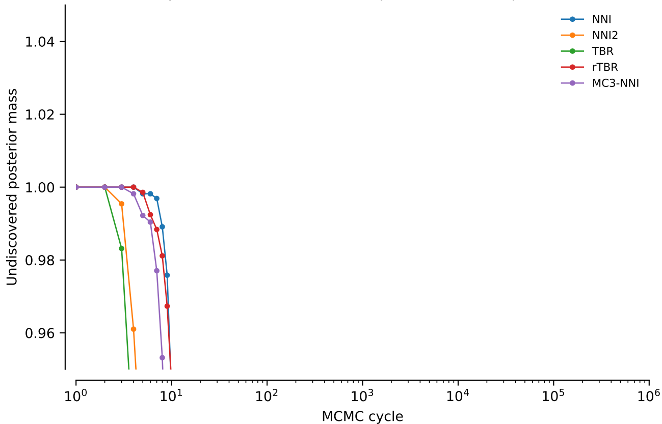
vert.atpase6.tw5: Undiscovered posterior mass: power = 0.2
