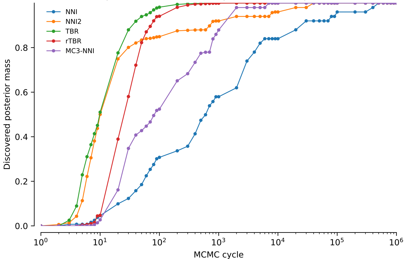
vert.atpase6.tw5: Discovered posterior mass: power = 0.3
