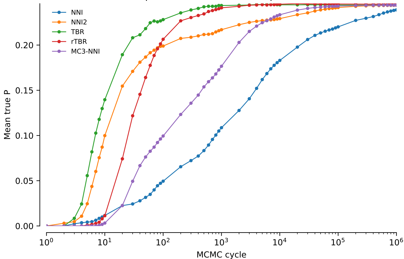
vert.atpase6.tw5: Mean true P: power = 0.3
