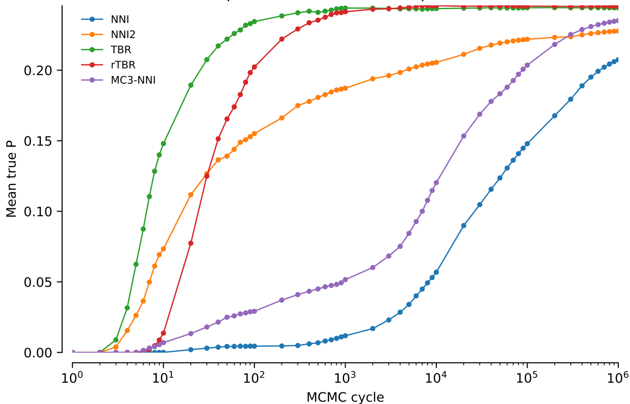
vert.atpase6.tw5: Mean true P: power = 0.4
