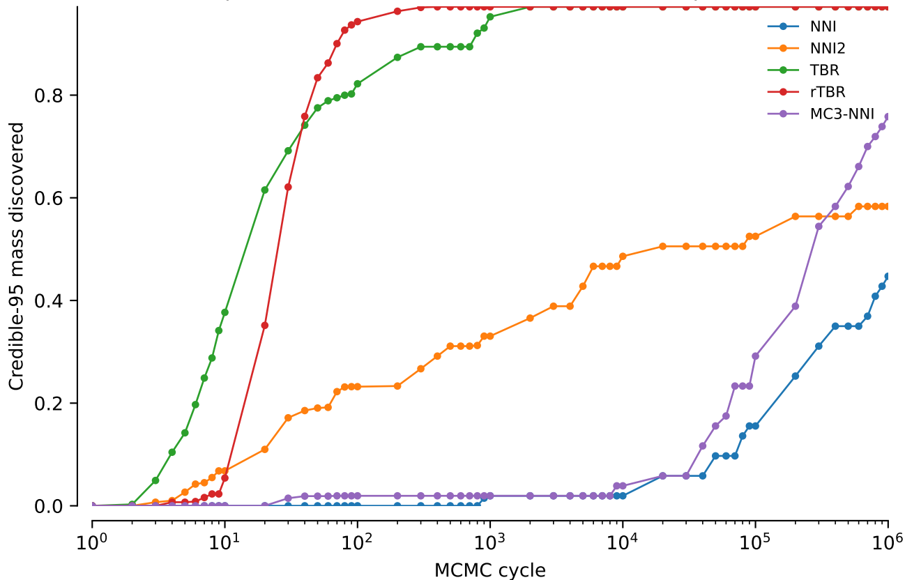
vert.atpase6.tw5: Credible-95 mass discovered: power = 0.5
