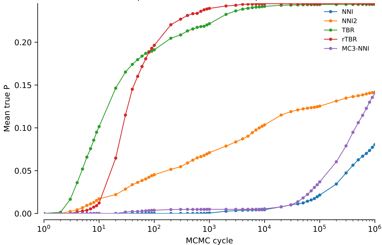
vert.atpase6.tw5: Mean true P: power = 0.5
