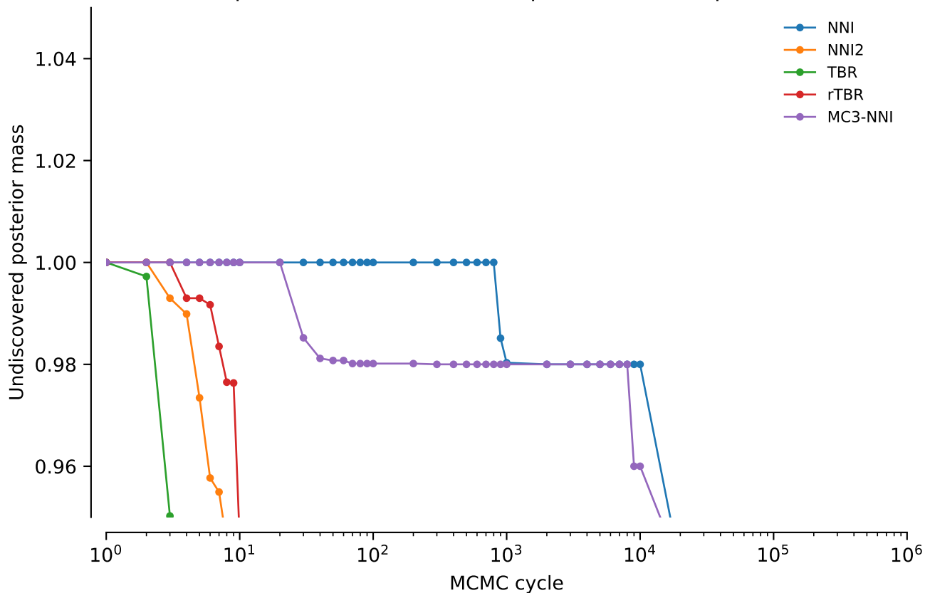
vert.atpase6.tw5: Undiscovered posterior mass: power = 0.5
