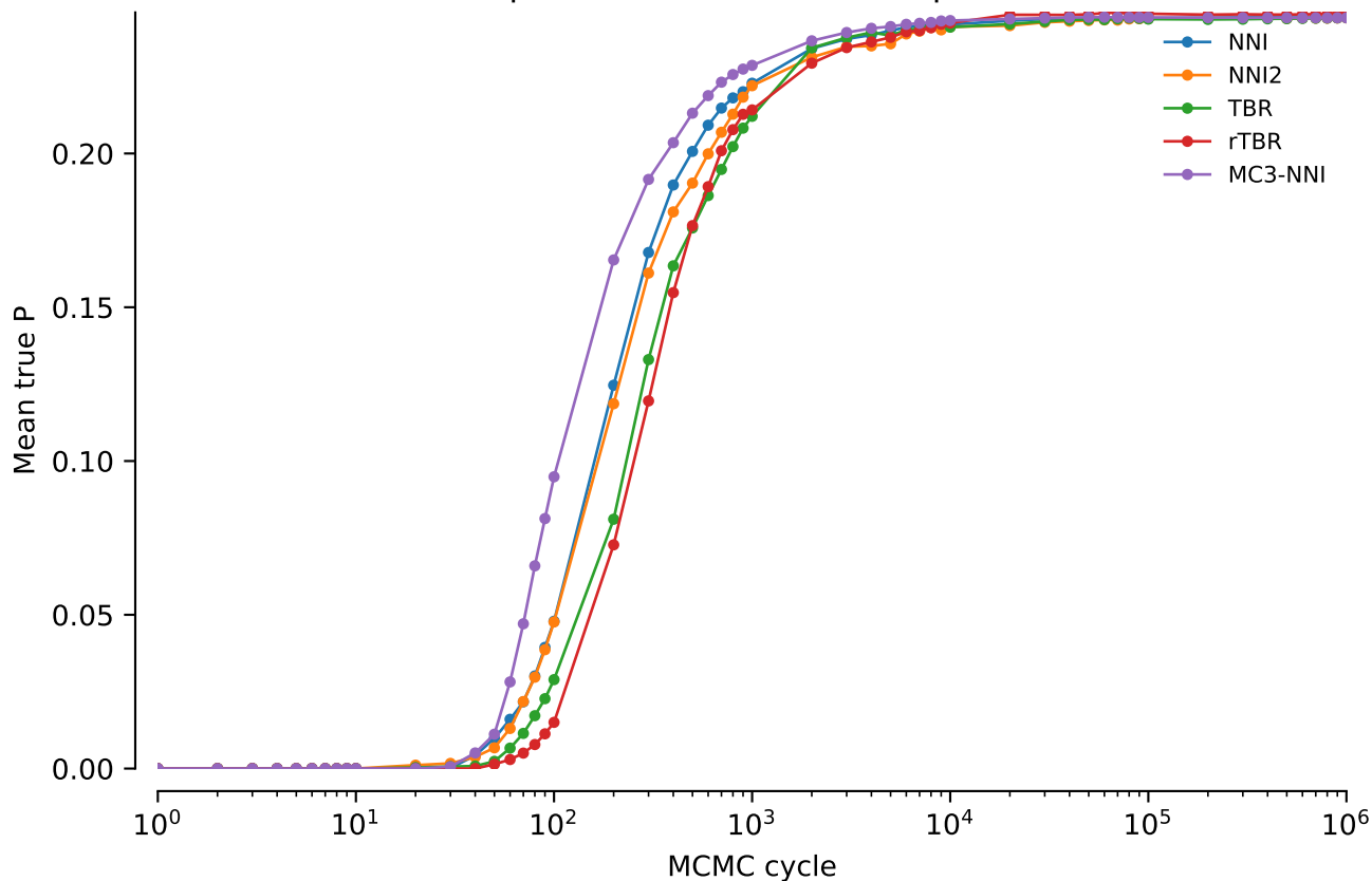
vert.atpase6.tw5: Mean true P: power = 0
