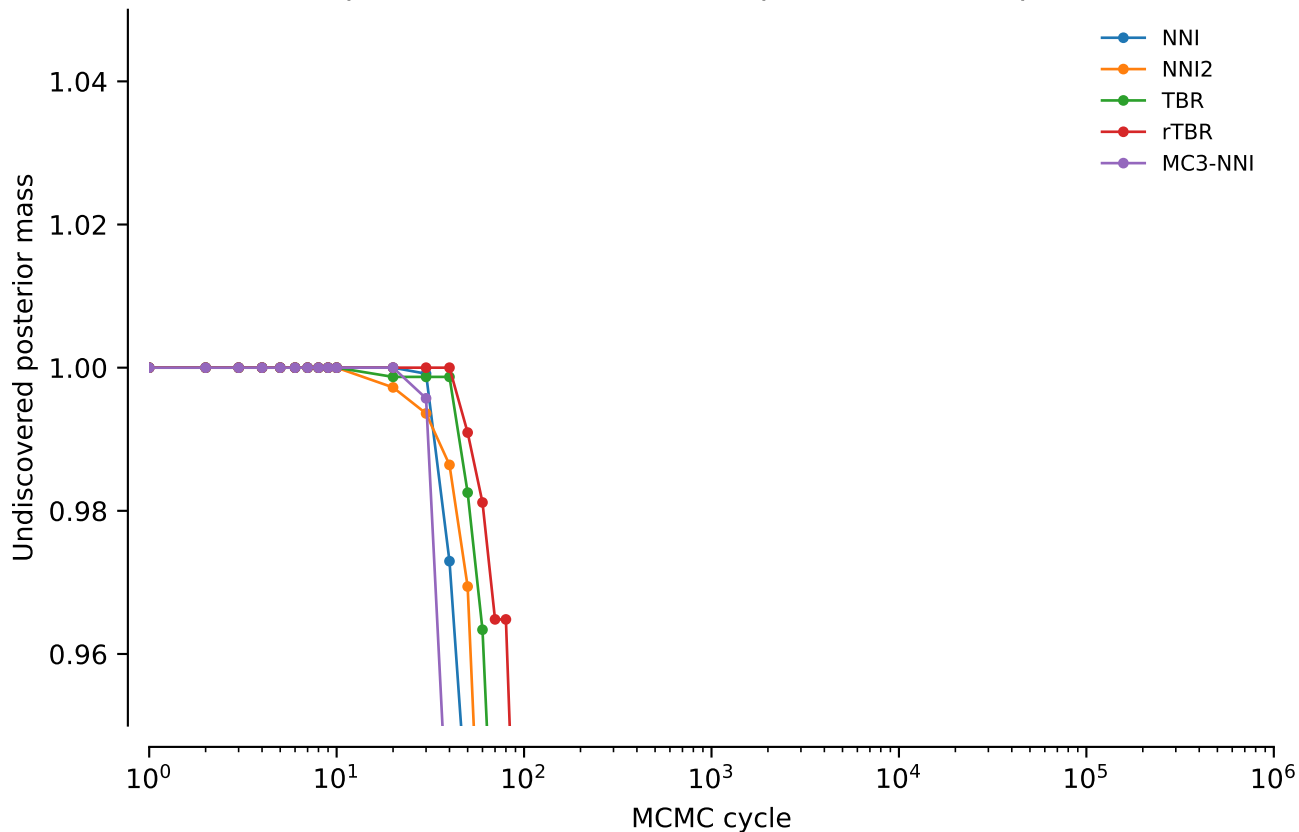
vert.atpase6.tw5: Undiscovered posterior mass: power = 0
