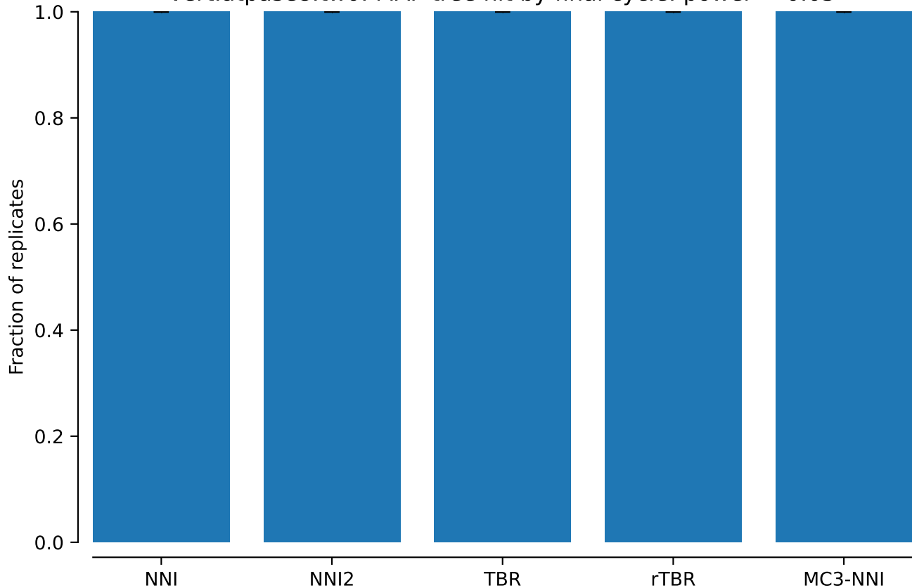
vert.atpase8.tw0: MAP tree hit by final cycle: power = 0.05
