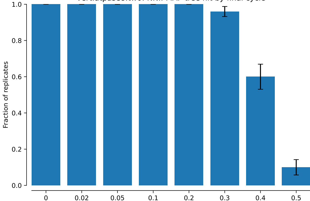
vert.atpase8.tw0: NNI: MAP tree hit by final cycle
