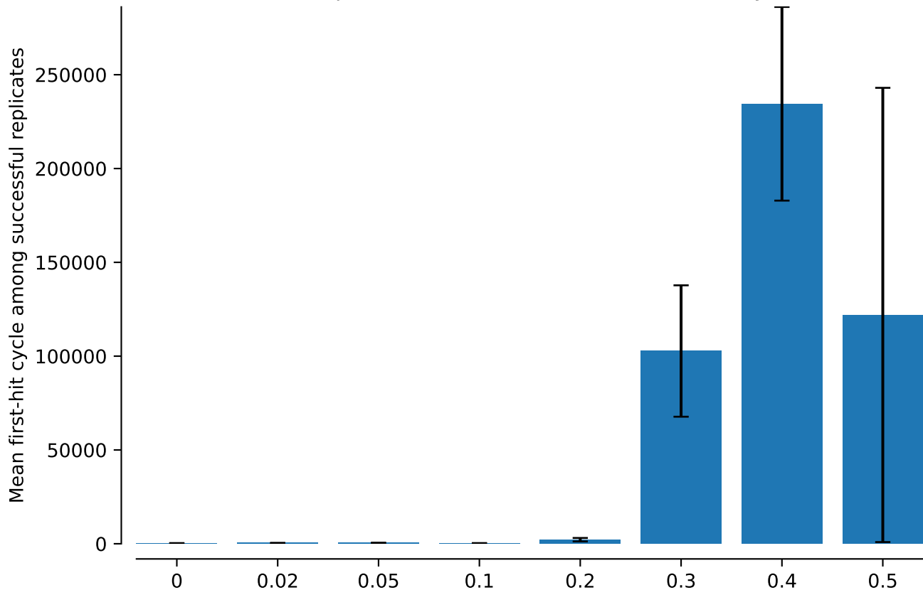
vert.atpase8.tw0: NNI: mean MAP first-hit cycle
