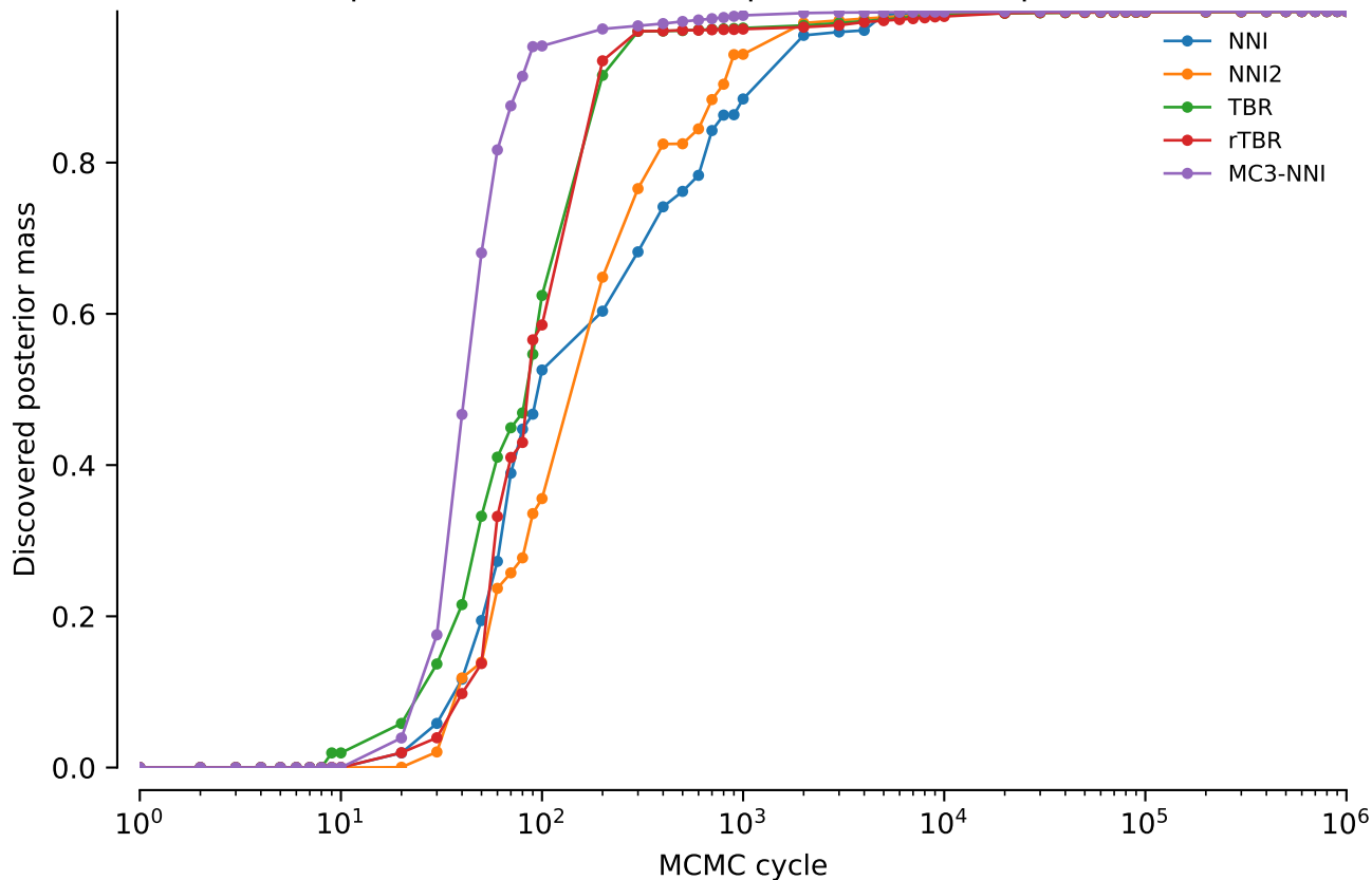
vert.atpase8.tw0: Discovered posterior mass: power = 0.02
