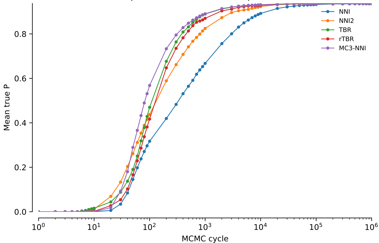
vert.atpase8.tw0: Mean true P: power = 0.05
