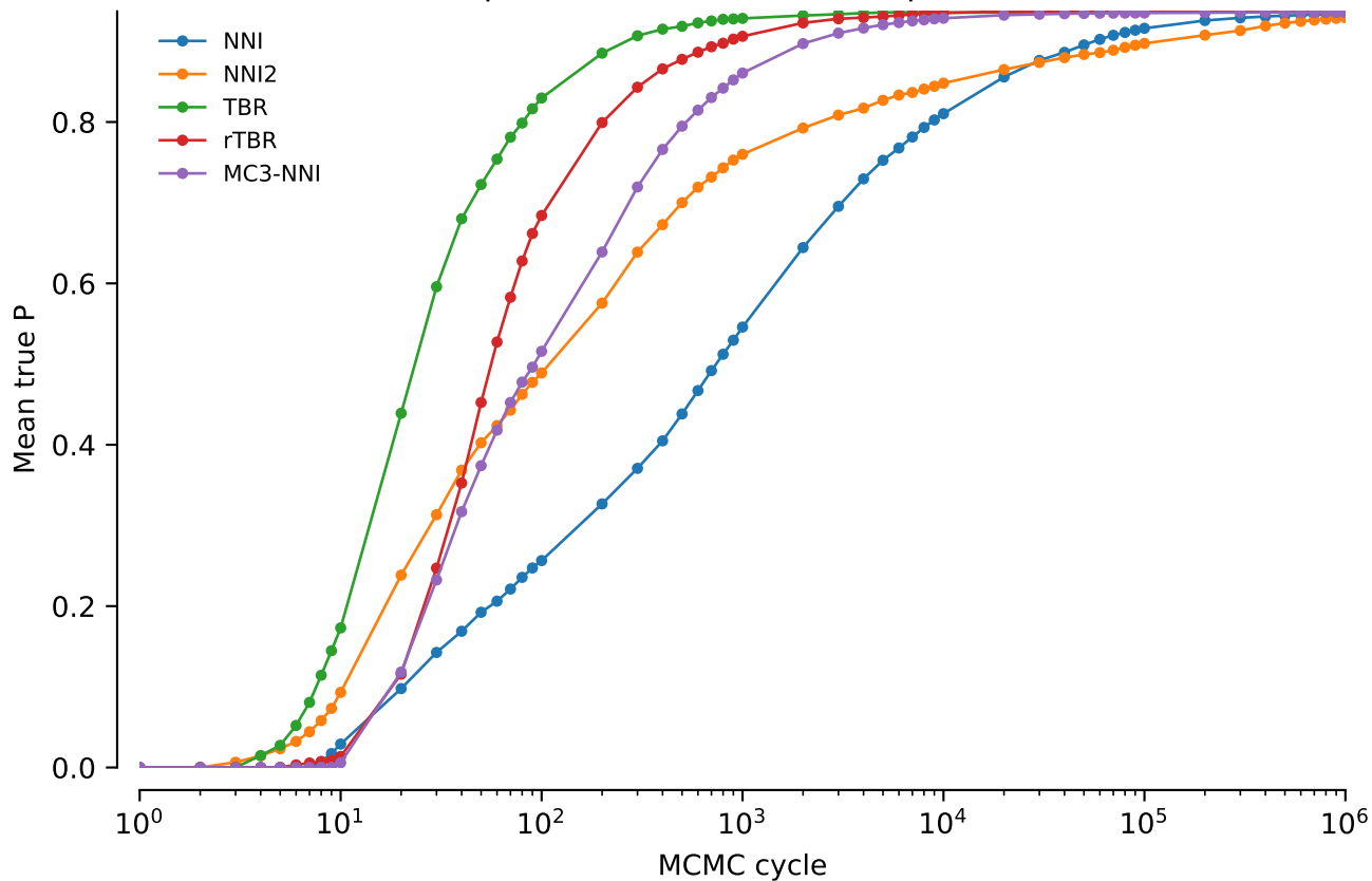
vert.atpase8.tw0: Mean true P: power = 0.2
